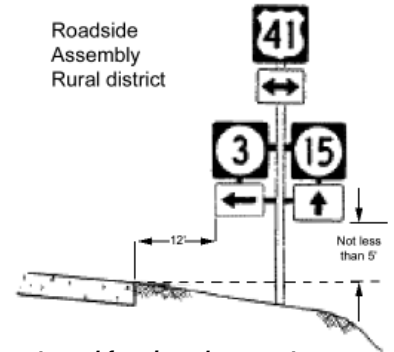
An example of a U-channel post used for sign placement and installation.
